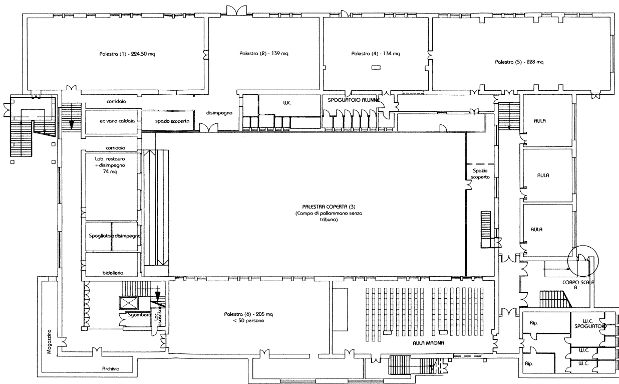
PIANTA PIANO SEMINTERRATO 1:250
